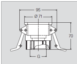
Quick-fit pipe connection (female thread)
