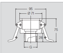
Quick-fit pipe connection (male thread)
